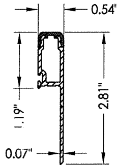
15 SILL RISER 356-A51-DP70
