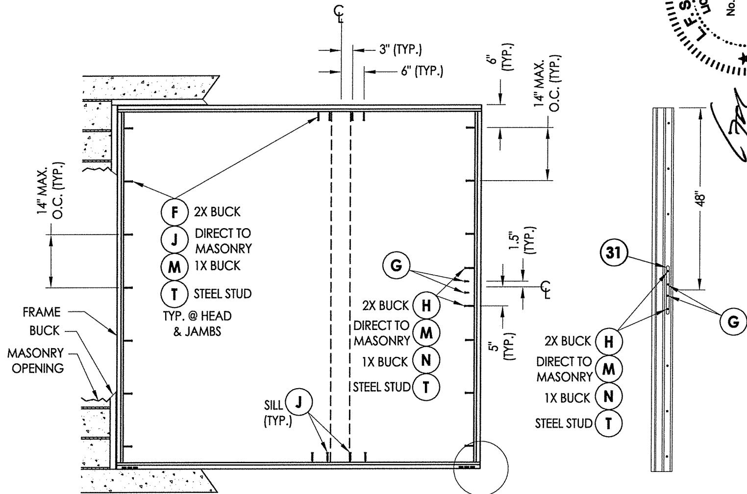
FRAME ANCHORING
