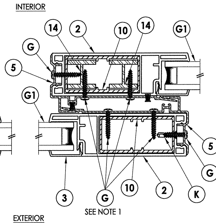
2 2 HORIZONTAL CROSS SECTION
